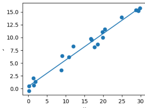
Fig. 4: A plot of a simple linear regression.
